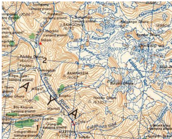
Fig.1:-Map of Region
