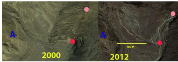
Fig.5:-Terminus closeup in Google Earth
