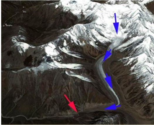
Fig.2:-Google Earth Image, blue arrows glacier flow, red arrow terminus.
