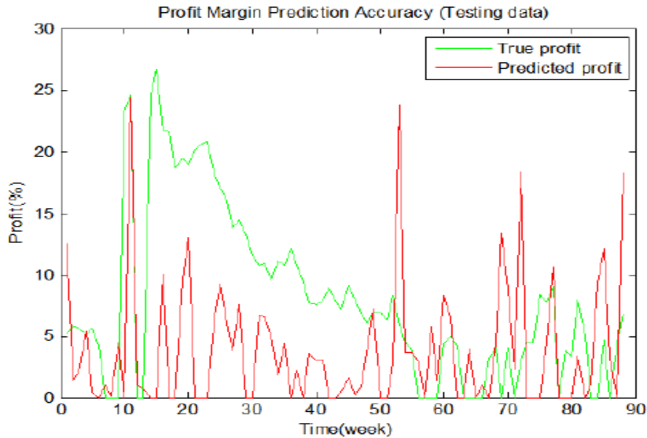
Fig. 9. Profits from the perfect Buys and Sells and profits predicted by the trained Neural Network (MSE=11.6%, Corr.Coeff.=0.11).
