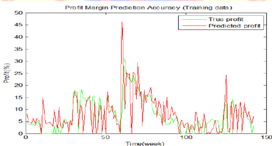
Fig. 6. Profits from the perfect Buys and Sells and profits predicted by the trained Neural Network. (MSE=8.7%, Corr.Coeff.=0.66)
