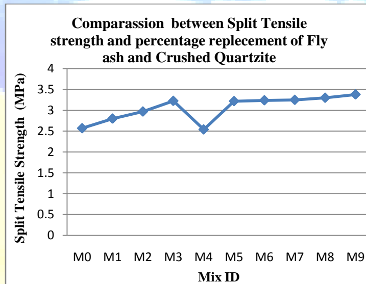
Figure 2: Mix ID vs Split Tensile Strength
