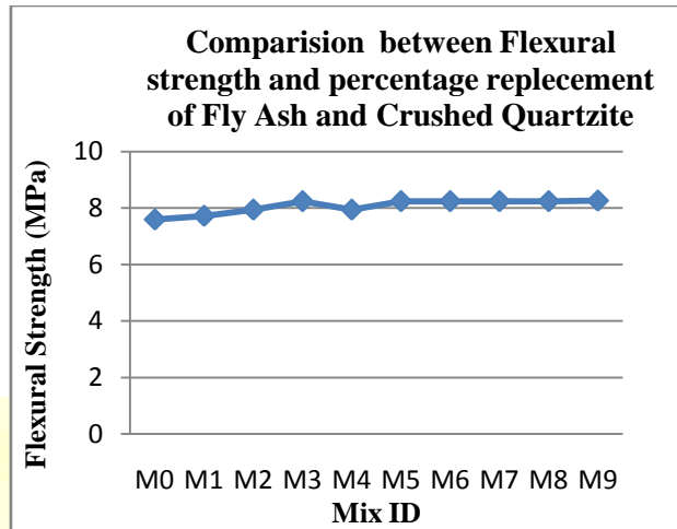
Figure 3: Mix ID vs Flexural Strength
