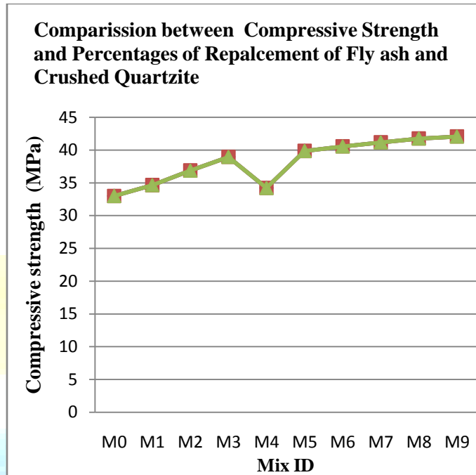
Figure 1: Mix ID vs Compressive Strength
