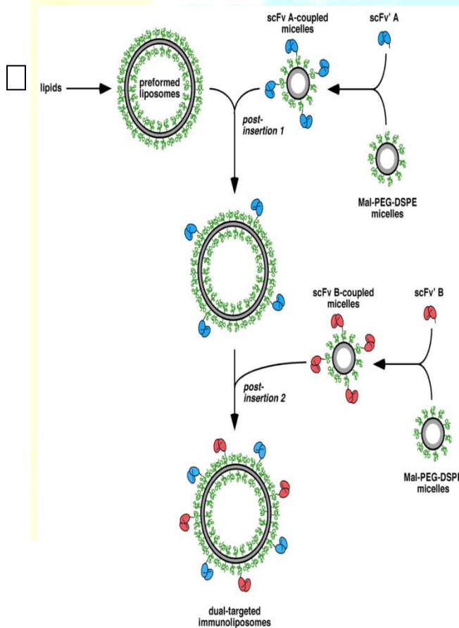
Figure1: Immunoliposomes
