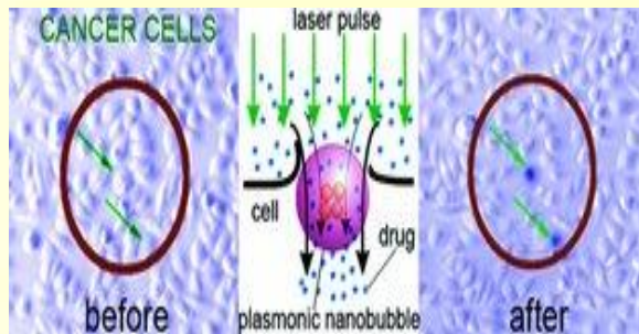
Figure 2: Nanobubbles
