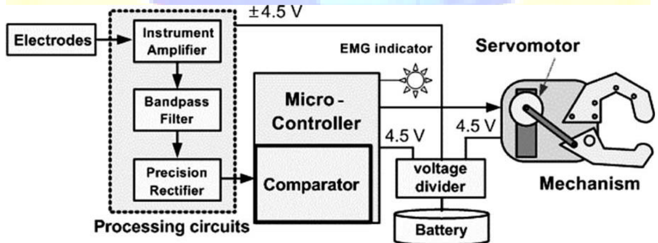
Fig. 4 Block presentation of proposed designed prosthetic arm
