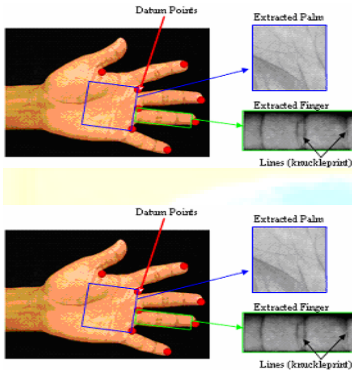
Figure 6: Extracted features
