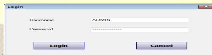
Fig.13 Login interface
