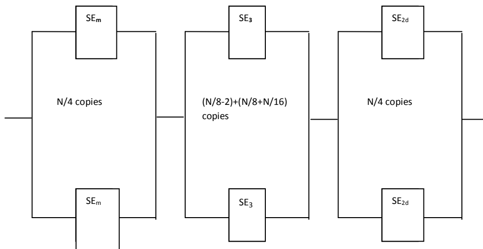
Fig 1:Upper Bound Reliability diagram of Triangle Network
