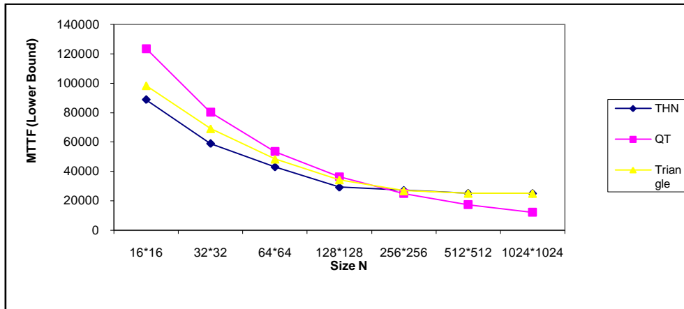
Fig 4: Comparison of Lower Bound MTTT of Triangle MIN with THN, QT Networks
