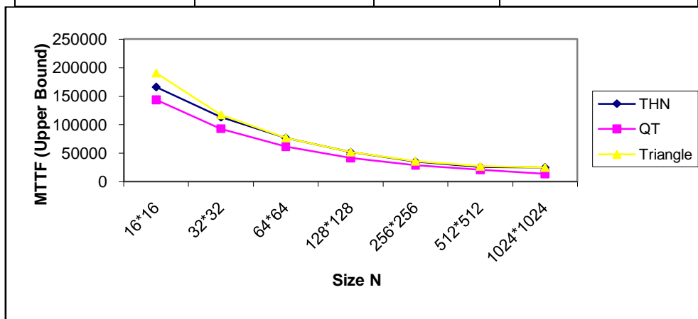
Fig 3: Comparison of Upper Bound MTTF of Triangle MIN with THN, QT Networks
