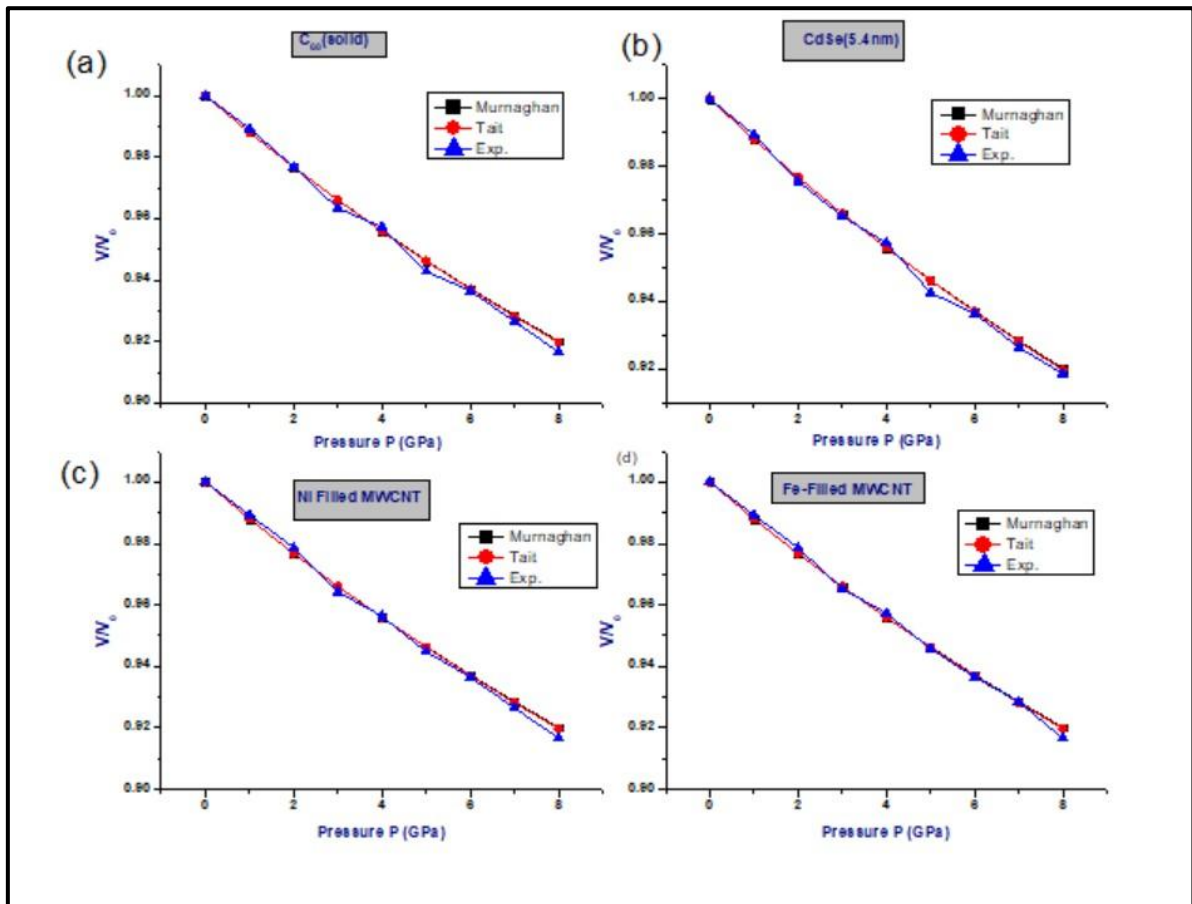
Figure 1. Variation of V/V_0 with pressure for (a) C_{60} (solid) with Exp. [15] (b) CdSe (5.4 nm) with Exp.[16] (c) Ni-Filled MWCNTs with Exp.[17] (d) Fe-filled MWCNTs with Exp.[18]
